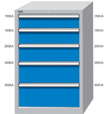
SPL-870-10 870Lx725Wx1200H
