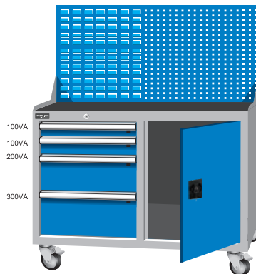
SPLW-011DM 1100Lx572Wx825H+500
